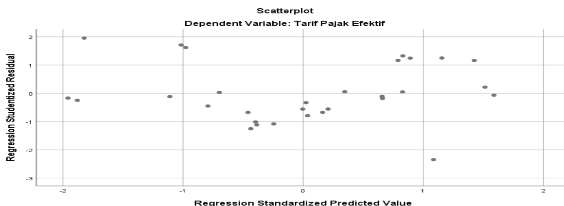
Figure 2. Heteroscedasticity Test Results
